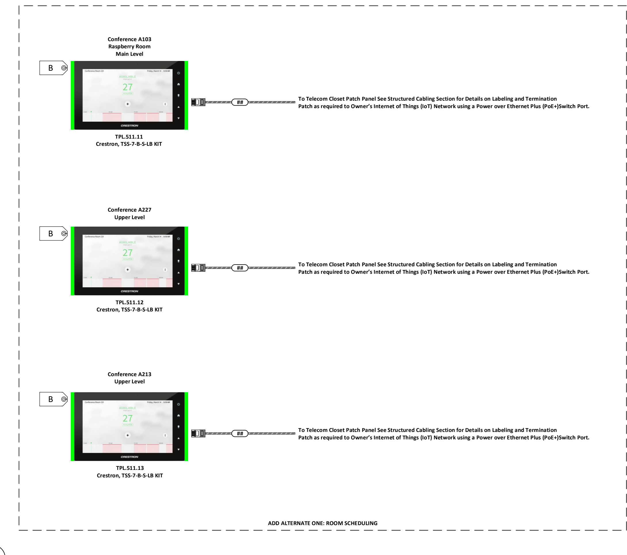
1 City Hall Room Scheduling Touch Panels
